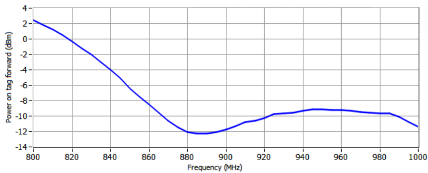
Sensitivity
