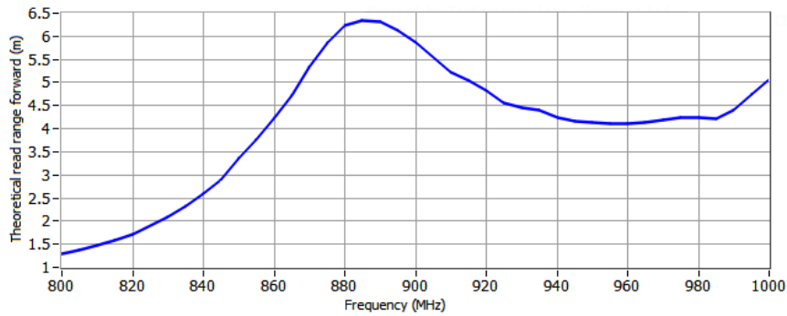
Read range
